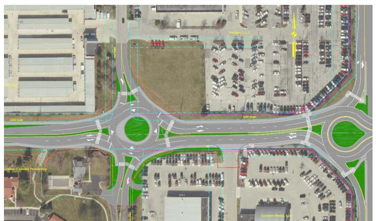
126th Street and Ford Drive Roundabout Project Rendering
